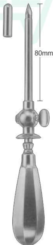
ROBERTS Inside diam. Outside diam. S12-138-50 4,0mm 5,0mm S12-138-60 5,0mm 6,0mm S12-138-65 5,5mm 6,5mm for abdominal puncture, with stop-cock
