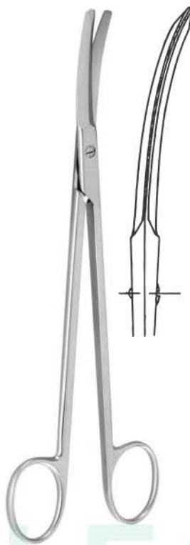
Potts-Smith Scissors S3-264-19 19 cm Blunt/Blunt Curved
