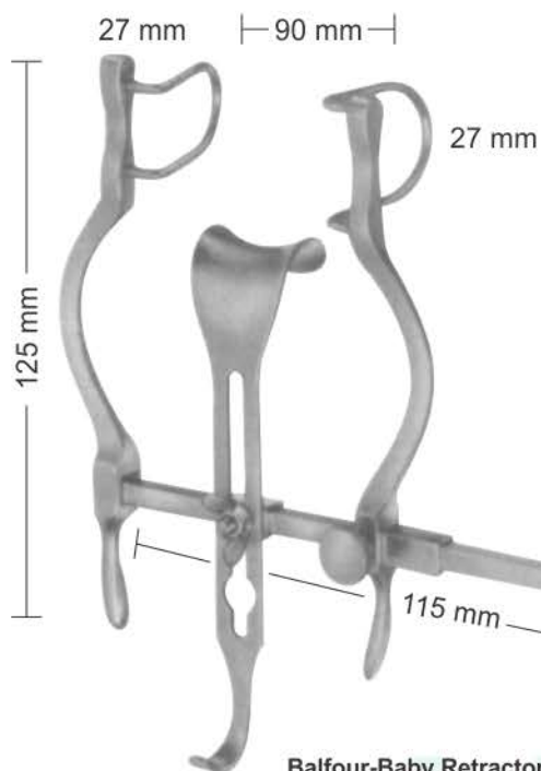
Balfour-Baby Retractor S11-746-00 Lateral Blades 27 mm deep Center blade 21 x 24 mm
