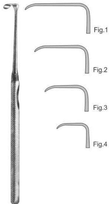
Mannerfelt-Langenbeck Retractors 15.5cm S11-121-01 15 x 6 mm Fig.1 S11-121-02 20 x 6 mm Fig.2 S11-121-03 25 x 6 mm Fig.3 S11-121-04 30 x 8 mm Fig.4
