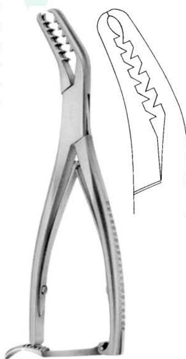
Semb Bone Holding Forceps S15-682-20 20.3cm with ratchet curved sideways deep teeth
