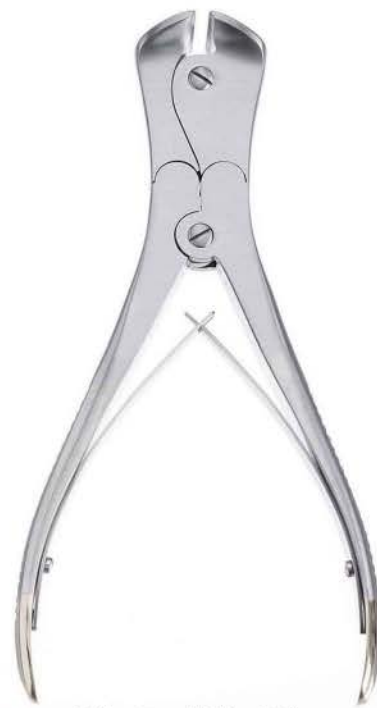
S Line Front Wire Cutter S15-901-22 22cm for hard wires up to 2.2mm, for soft wires up to 3mm tungsten carbide inserts
