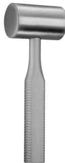
Heath Mallets S15-094-40 18cm 40mmØ - 700g S15-094-45 20cm 45mmØ - 1000g Lead filled
