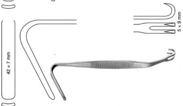
Item Code Description LP-472 AUFRICHT WALTER NASAL RETRACTOR, 13.5CM, DOUBLE ENDED, SHARP, 42X7MM
